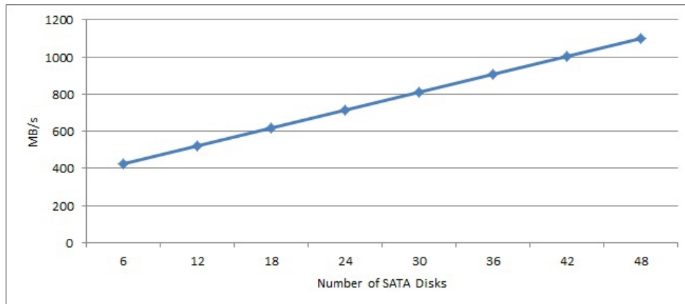
Figure 6. ReadyDATA 5200 SATA drive sustained throughput
