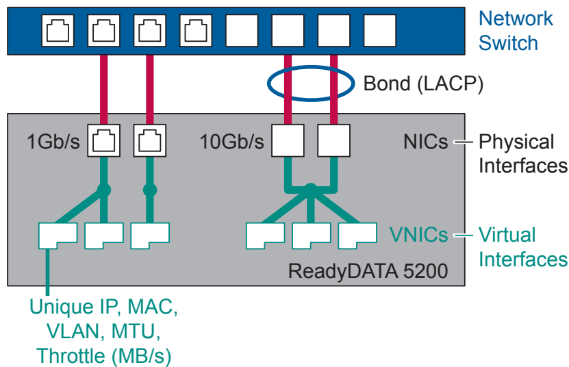
Figure 5. Virtual network interfaces
